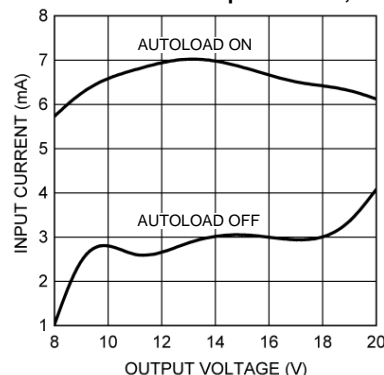
Autoload Effect on Input Current, No Load
