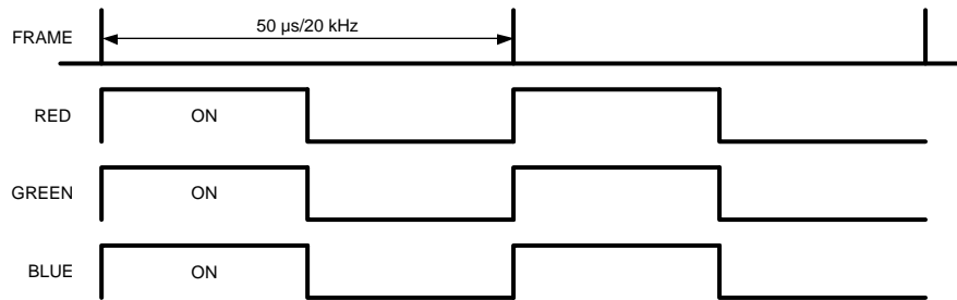
Figure 5. Overlapping Mode
