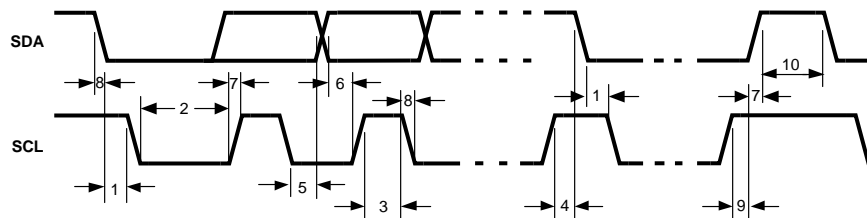
Figure 18. I²C Timing Diagram
