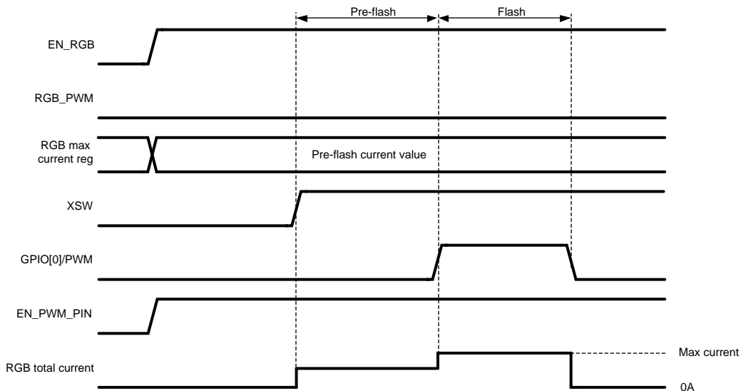
Figure 9. Using Flash Mode
