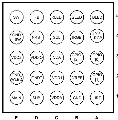
Figure 2. 25-Bump Thin Micro SMD Package, Large Bump Bottom View
