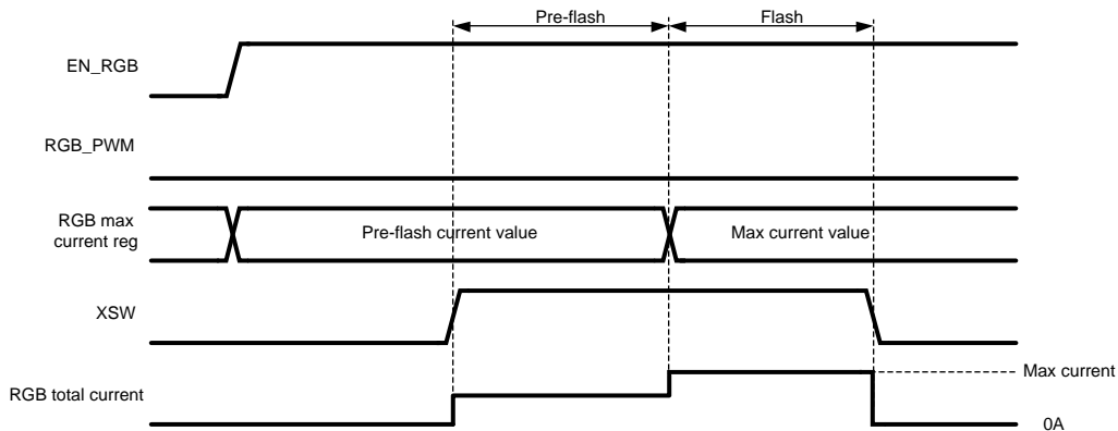
Figure 8. Controlling RGB Max Current Values to Introduce Flash
