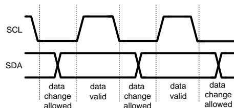
Figure 13. I 2 C Signals: Data Validity
