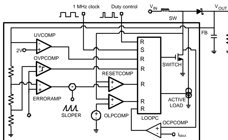
Figure 3. Boost Converter Topology
