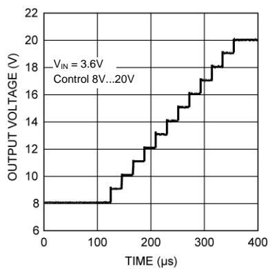
Figure 4. Boost Output Voltage Control
