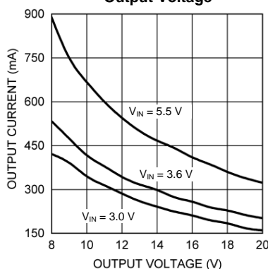
Boost Maximum Current vs. Output Voltage
