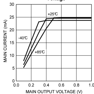
WLED Output Current vs. Voltage
