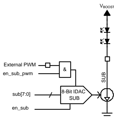
Figure 11. SUB output for 2 LEDs (DISPL = 0)
