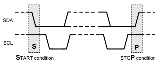
Figure 14. I 2 C Start and Stop Conditions
