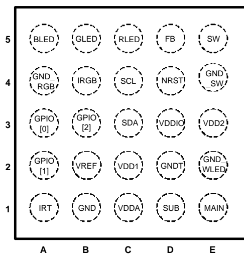
Figure 1. 25-Bump Thin Micro SMD Package, Large Bump Top View
