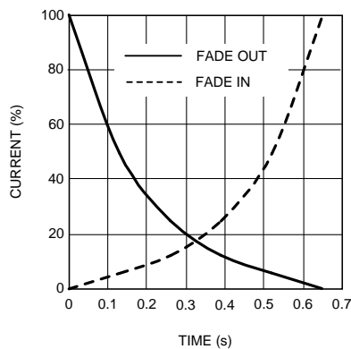
WLED Dimming, SLOPE=0
