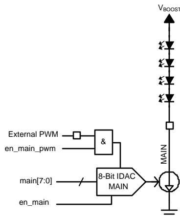
Figure 10. MAIN output for 4 LEDs (DISPL = 0)
