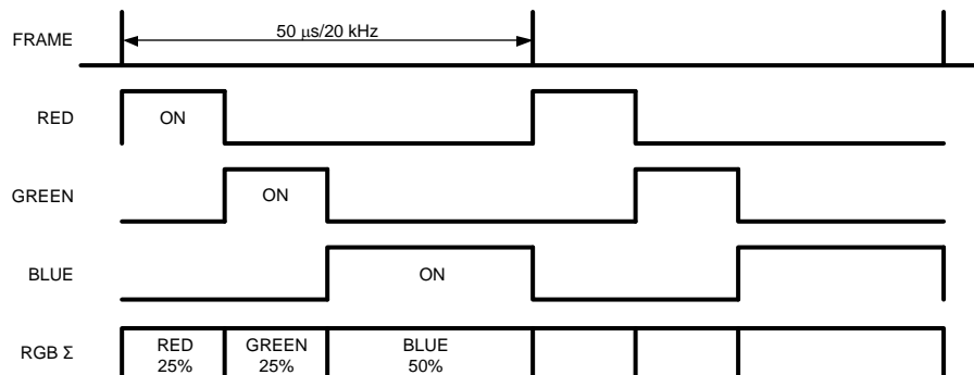
Figure 6. Non-Overlapping Mode
