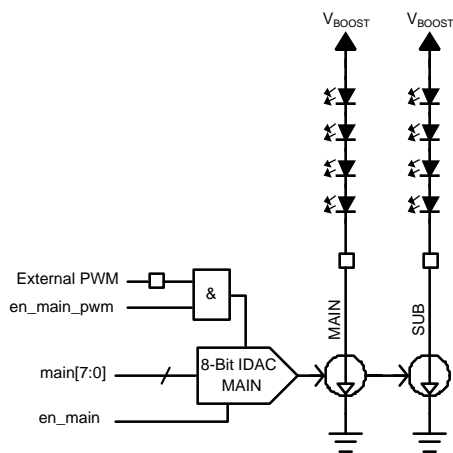
Figure 12. MAIN and SUB outputs for 8 LEDs (DISPL = 1)
