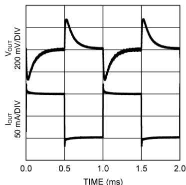
Boost Load Transient Response 50mA – 150mA
