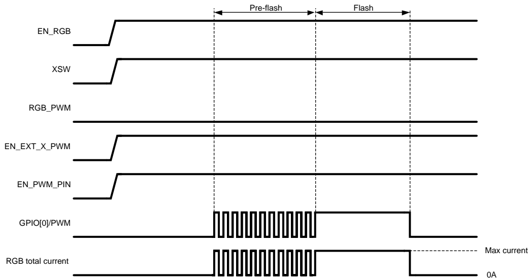
Figure 7. Using External PWM Control for Flash
