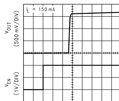
Enable Start-Up Time ( V_{OUT} = 1.8V )
