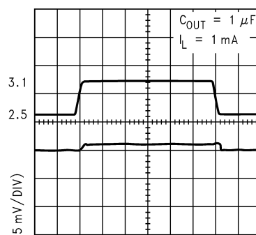
Line Transient Response (1.5V V_{OUT} )
