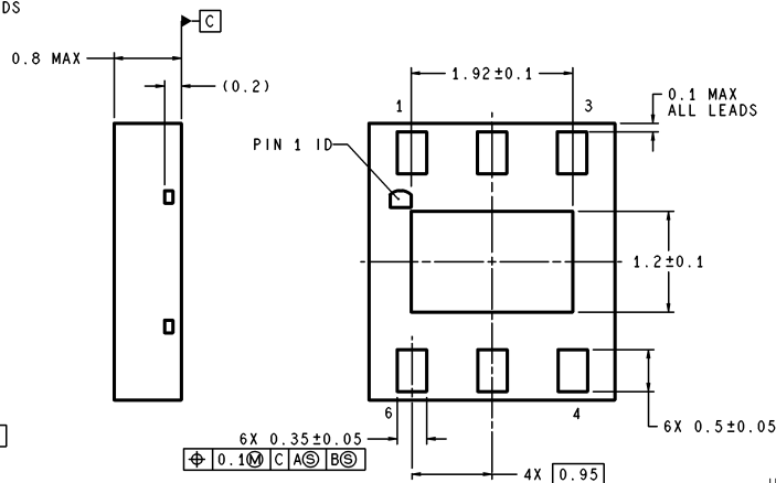
LLP, 6 Lead, Package (SOT23 Land) NS Package Number LDE06A
