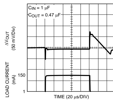
Figure 16. Load Transient
