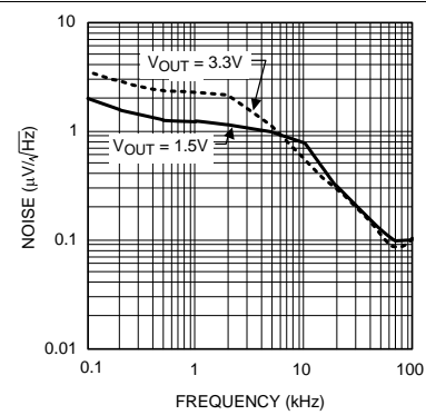
Figure 12. Noise Density
