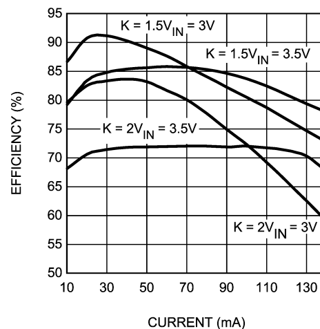
Charge Pump Efficiency vs Load Current
