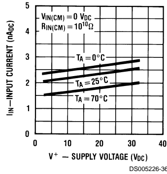
Input Current
