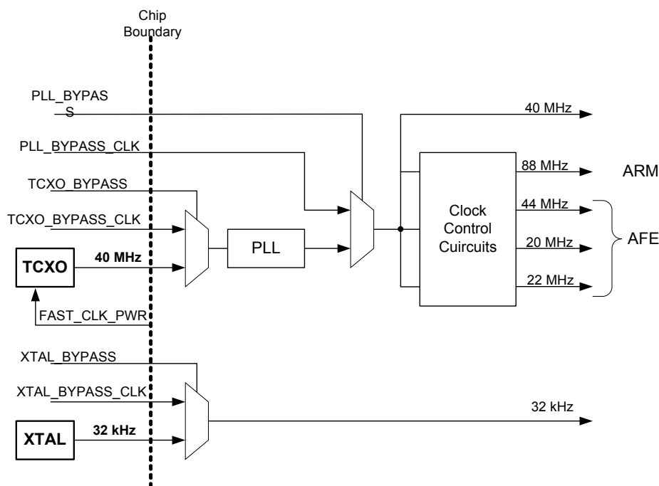
Figure 3. LP1072 Clocks
