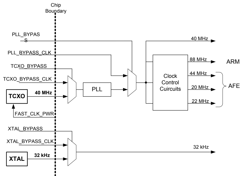
Figure 3. LP1071 Clocks
