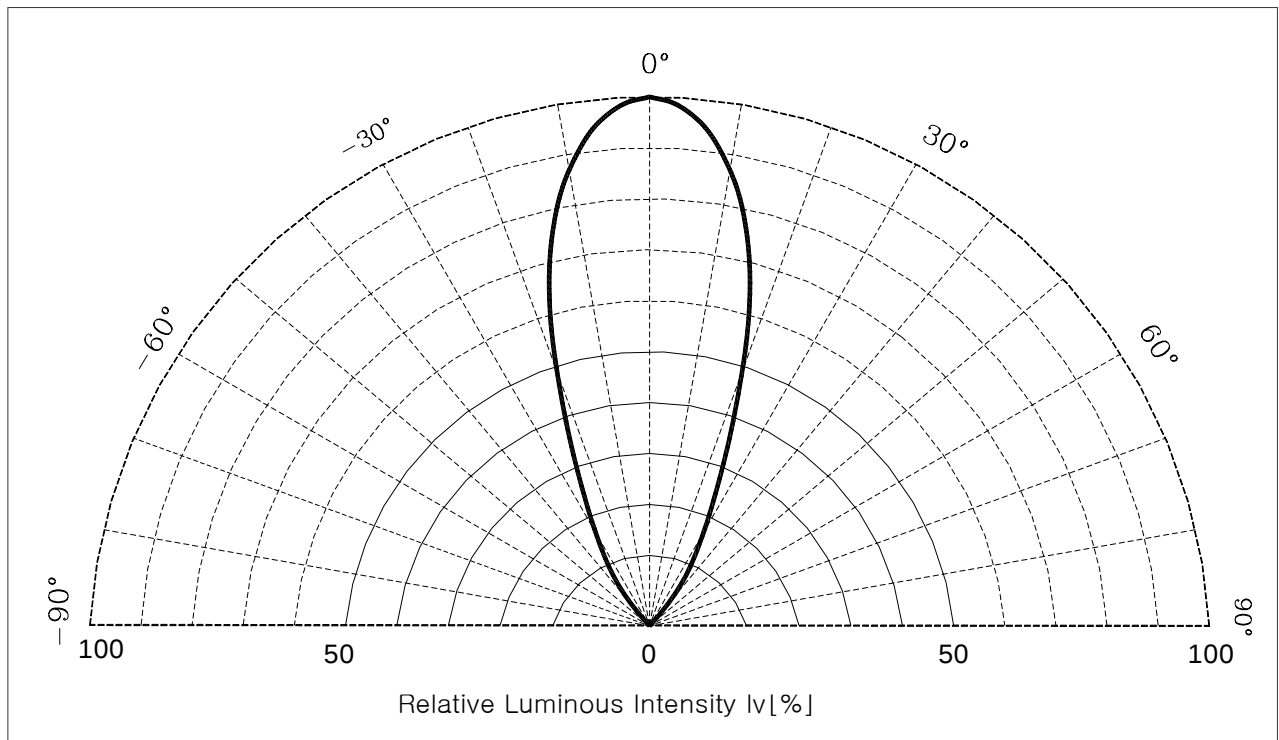
Fig. 6 Radiation Diagram
