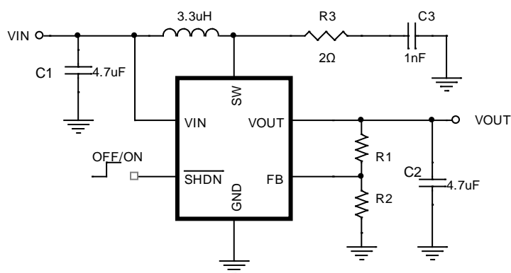
Figure 3. Vin>4.5V
