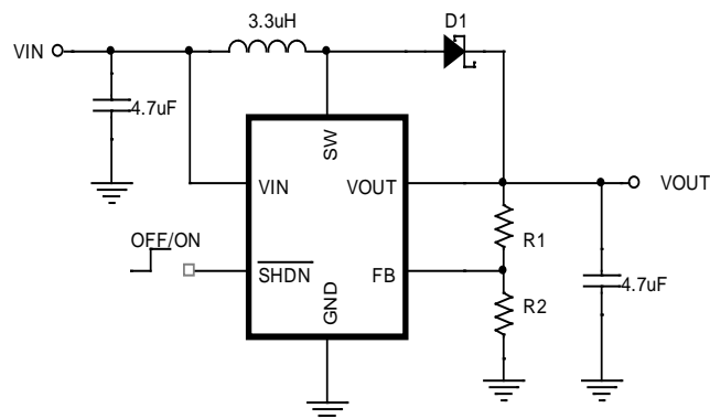
Figure 2.Vout>4.5V
