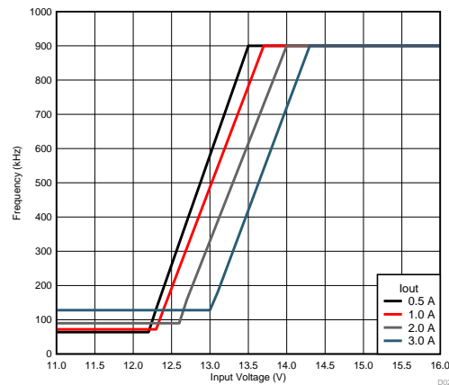
Figure 23. Frequency Foldback
