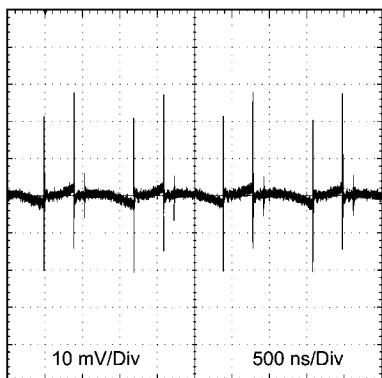
Output Ripple 12V_{IN} 3.3V_O @ 5A BW = 250\text{ MHz}
