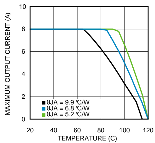
Figure 51. Thermal Derating Curve
