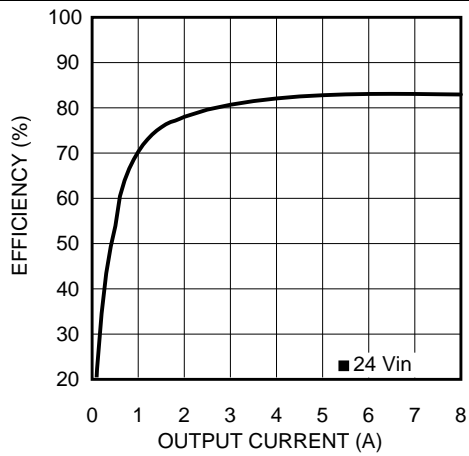
Figure 50. Efficiency
