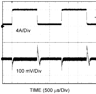
Transient response 12V_{IN} , 1.2V_{OUT} 1 to 8A Step
