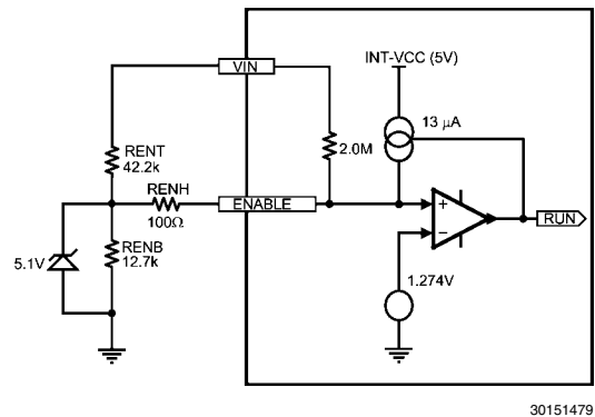
FIGURE 1. Enable input detail
