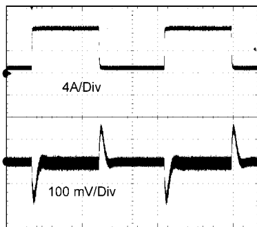
Transient response 12V_{IN} , 5.0V_{OUT} 1 to 8A Step
