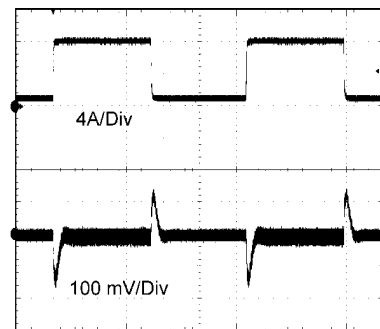
Transient response 12V_{IN} , 3.3V_{OUT} 1 to 8A Step
