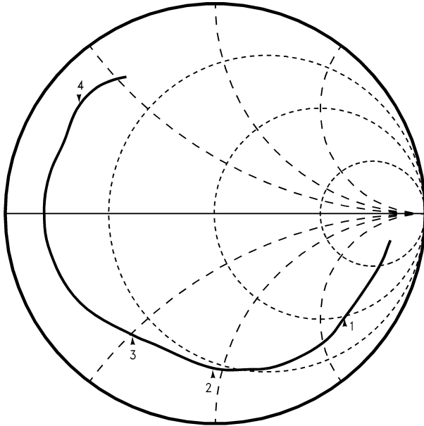
LMX243x UTCSP FinRF Input Impedance V CC = EN = 2.50V, T A = +25°C
