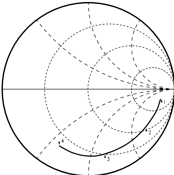
LMX243x UTCSP FinIF Input Impedance V CC = EN = 2.50V, T A = +25°C
