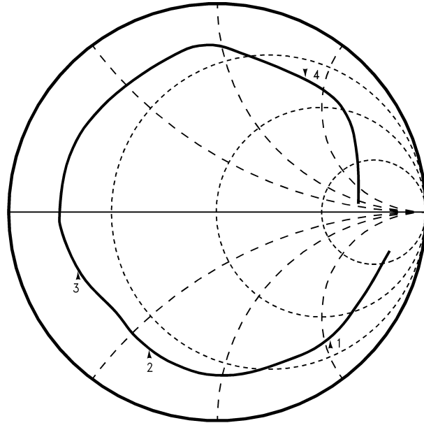
LMX243x TSSOP FinRF Input Impedance V CC = EN = 2.50V, T A = +25°C
