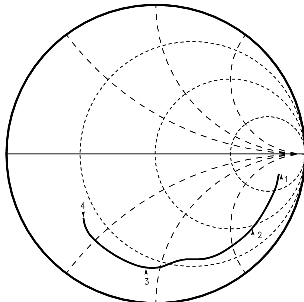
LMX243x TSSOP FinIF Input Impedance V CC = EN = 2.50V, T A = +25°C
