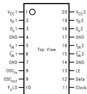
LMX2336U (Top View)
