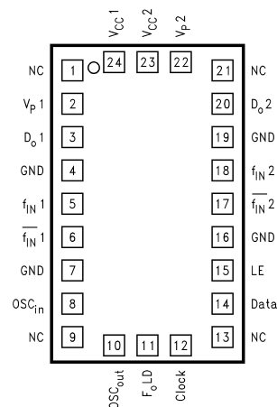
LMX2336U (Top View)
