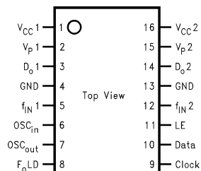
LMX2335U (Top View)
