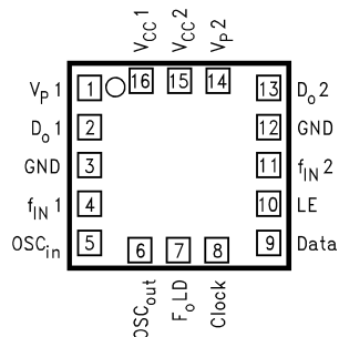
LMX2335U (Top View)
