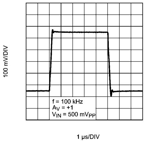
Large Signal Step Response with Gain = 1
