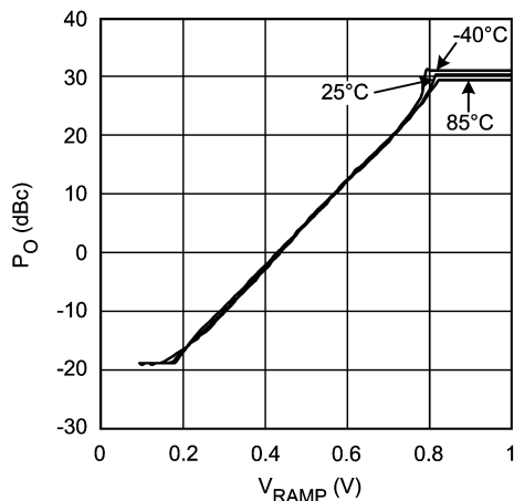
Closed Loop P_{OUT} (PA) vs. V_{RAMP} @ 1900MHz
