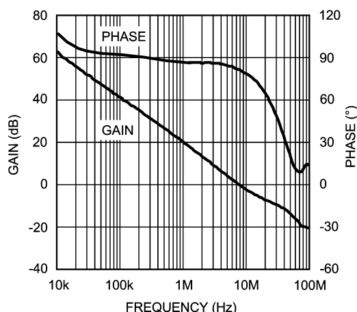
Gain and Phase vs. Frequency Error Amplifier
