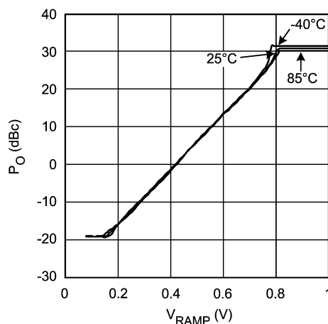
Closed Loop P_{OUT} (PA) vs. V_{RAMP} @ 1800MHz
