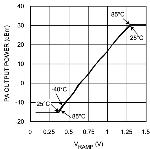
Closed Loop P_{OUT} (PA) vs. V_{RAMP} @ DCS 1800 MHz Band
