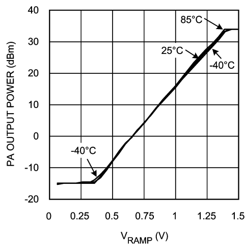
Closed Loop P_{OUT} (PA) vs. V_{RAMP} @ GSM 900 MHz Band
