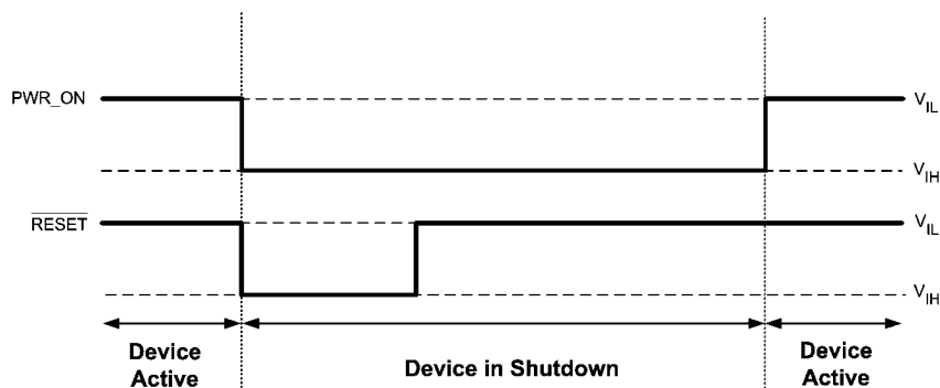
FIGURE 9. I²C Reset Timing Diagram
