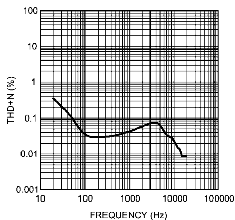
THD+N vs Frequency V_{DD} = 5\text{V} , P_{\text{OUT}} = 150\text{mW} Downlink Path
