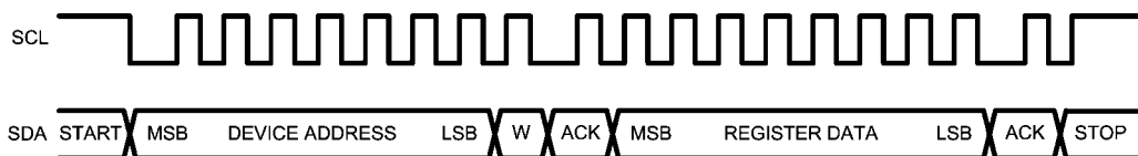
FIGURE 8. Start and Stop Diagram
