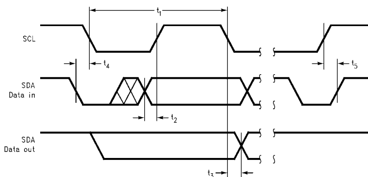
FIGURE 6. I²C Timing Diagram
