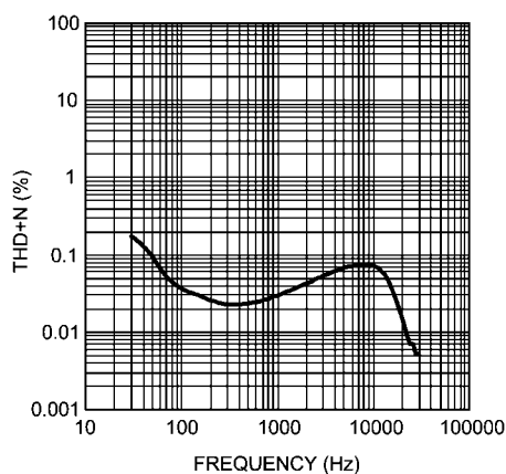
THD+N vs Frequency V_{DD} = 3.6\text{V} , P_{\text{OUT}} = 50\text{mW} Downlink Path
