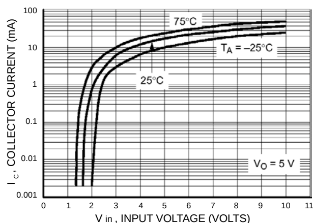
Figure 32. Output Current versus Input Voltage
