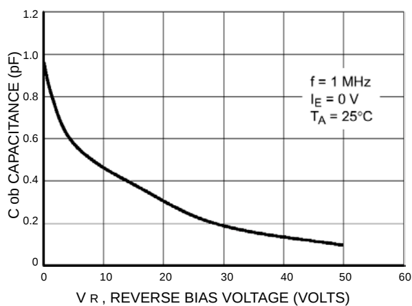
Figure 26. Output Capacitance
