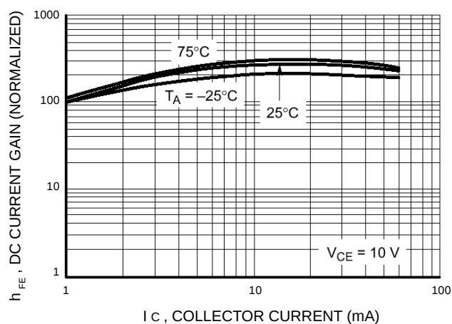
Figure 25. DC Current Gain
