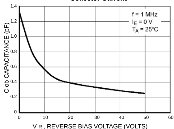
Figure 31. Output Capacitance
