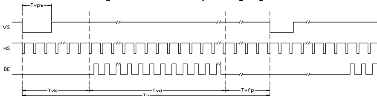
Figure 6-4-2 Vertical input timing diagram.
