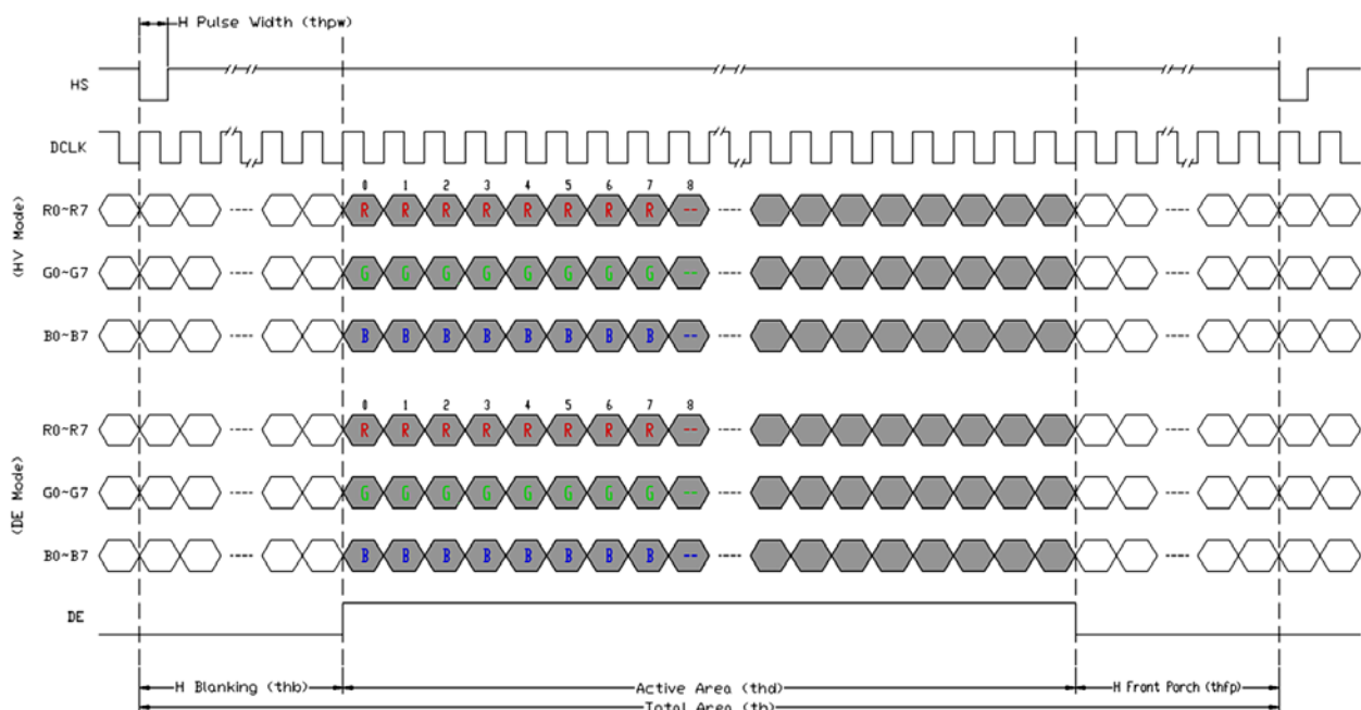
Figure 6-4-1 Horizontal input timing diagram.
