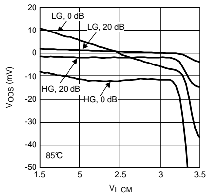
Figure 35. A_{V_{CM}}
