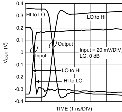
Figure 37. Step Response
