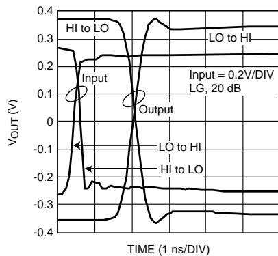
Figure 39. Step Response
