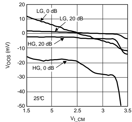
Figure 34. A_{V_{CM}}
