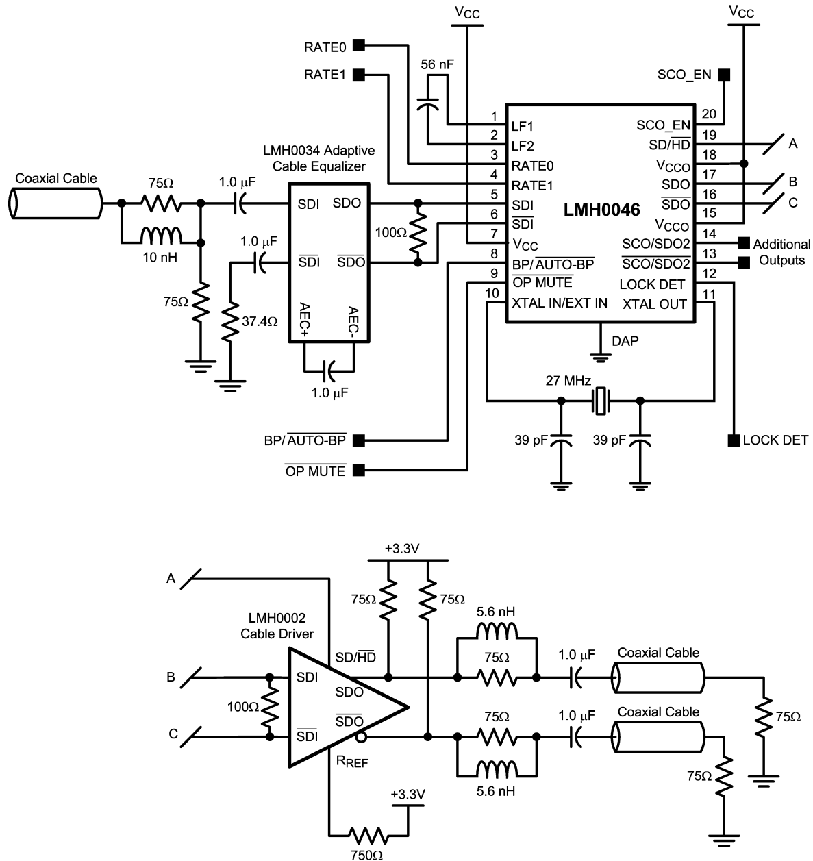
FIGURE 1. Application Circuit
