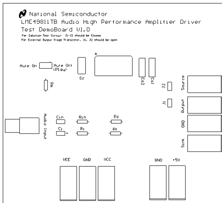
Silkscreen Layer
