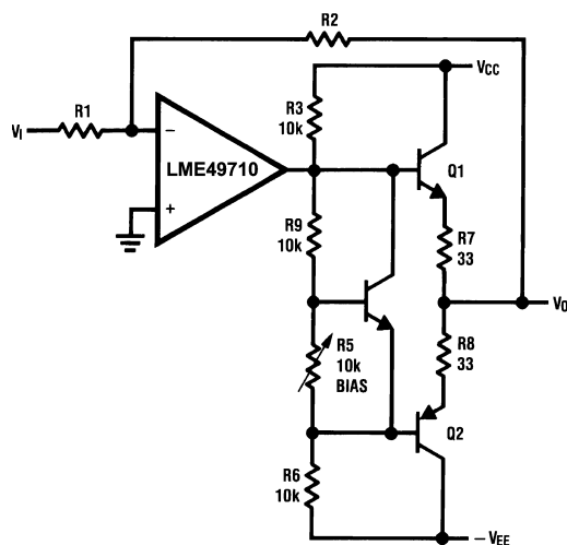
Figure 91. Line Driver
