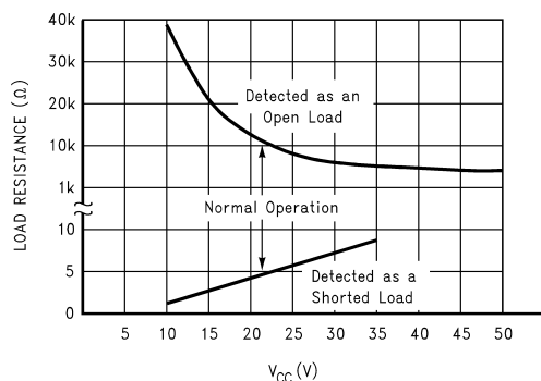
Figure 16. Load Resistance Detected as Errors
