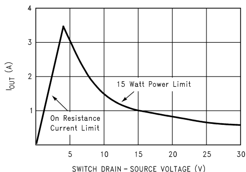
Figure 10. Maximum Output Current with Instantaneous Power Limiting
