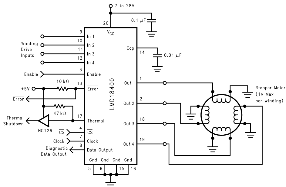
Figure 21. Unipolar Drive for a 4-Phase Stepper Motor
