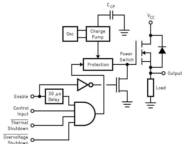
Figure 7. Control Logic for Each Power Switch
