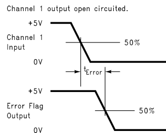
Figure 4. Error Reporting Delay
