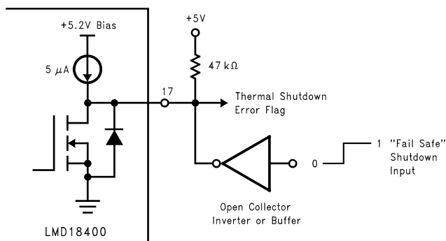
Figure 14. Thermal Shutdown Flag and Shutdown Input
