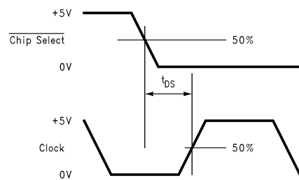
Figure 5. Data Setup Time
