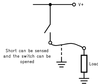
Figure 15. Detection Circuitry for Open/Shorted Loads
