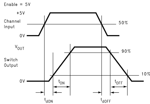
Figure 2. Switching Turn ON/OFF
