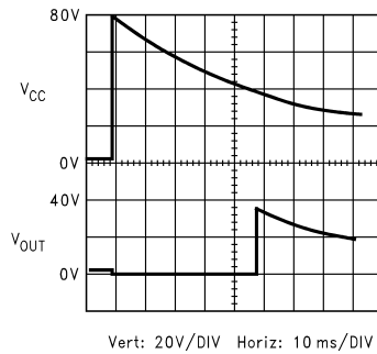
Figure 8. Overvoltage/Undervoltage Shutdown
