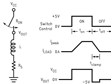
Figure 18. Switching an Inductive Load
