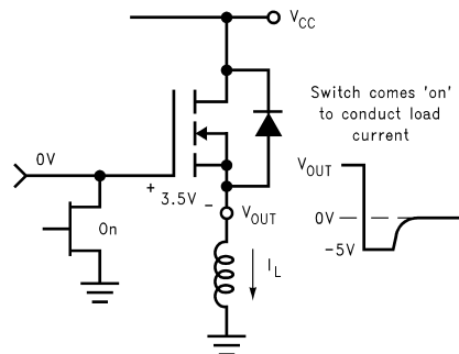
Figure 9. Turn-OFF Conditions with an Inductive Load
