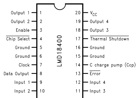
Figure 1. Order Number LMD18400N See NS Package Number N20A
