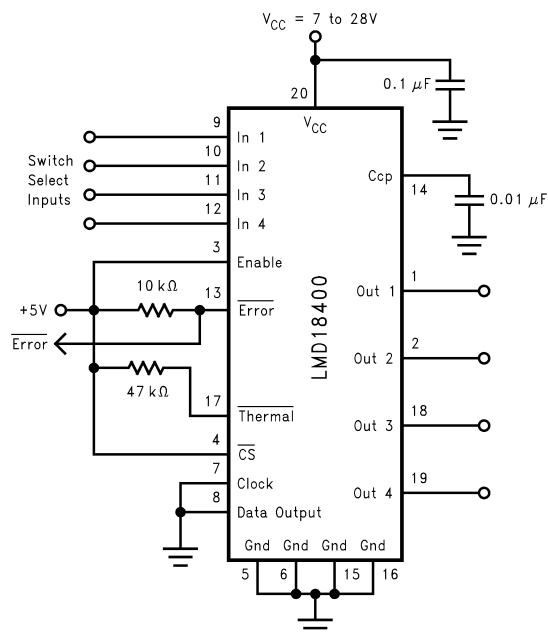
Figure 22. Recommended Connection If No Diagnostics are Required
