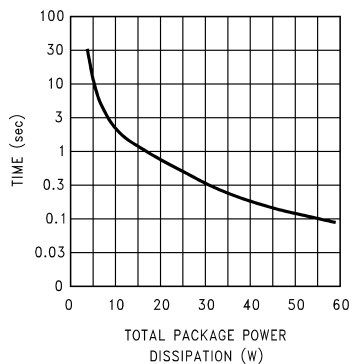
Figure 19. Approximate time required for the die to reach the 170°C thermal shutdown point from 25°C for different total package power dissipation levels.
