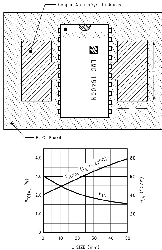
Figure 17. Maximum Power Dissipated and Junction to Ambient Thermal Resistance vs Size Recommended PC Board Layout to Reduce the Thermal Resistance from Junction-to-Ambient
