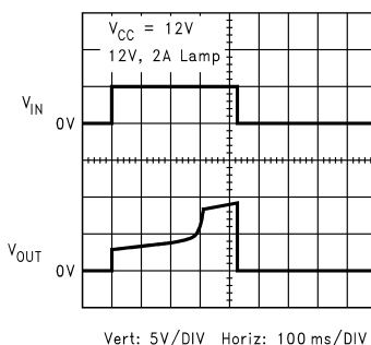
Figure 11. Driving a Lamp / Soft Turn-On of a Lamp Load
