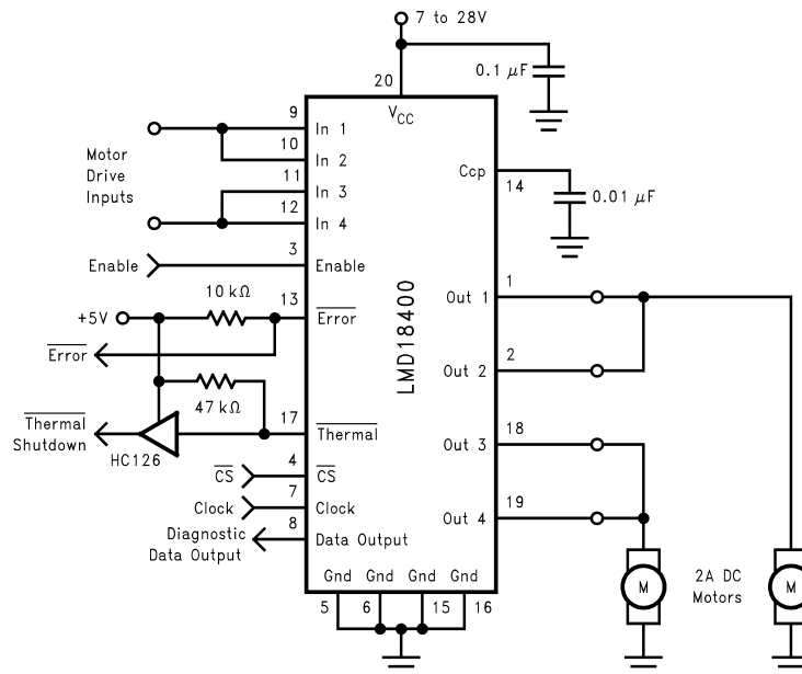
Figure 25. Paralleling switches for higher current capability. Positive temperature coefficient of the switch ON resistance provides ballasting to evenly share the load current between the switches. Any combination of switches can be paralleled. Required peak load current will depend upon the motor load. Motor speed control can be provided by a PWM signal of up to 20 kHz applied to the motor drive input lines.
