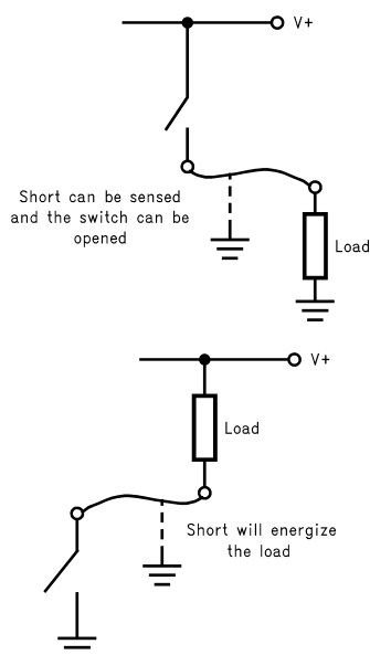
Figure 6. High-Side vs Low-Side Drive
