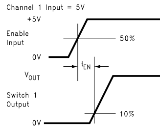
Figure 3. Enable Turn-On
