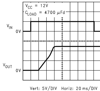
Figure 12. Driving a Large Capacitive Load
