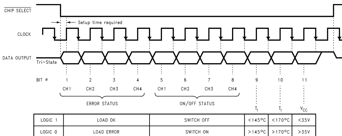
Figure 13. Serial Diagnostic Data Assignments
