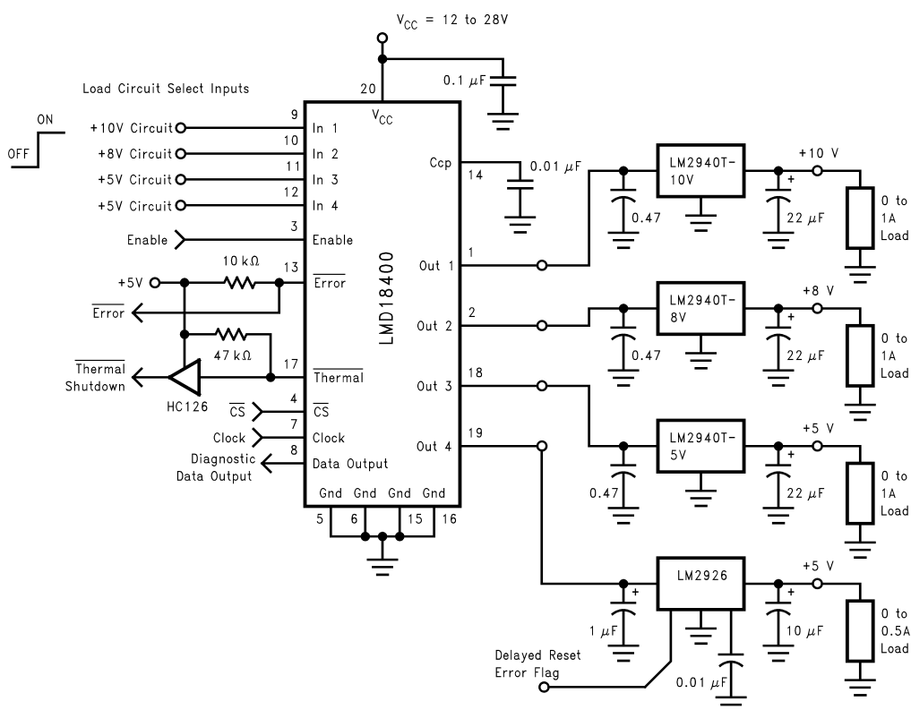
Figure 20. ON/OFF Switching of Multiple Voltage Regulated Circuit Loads
