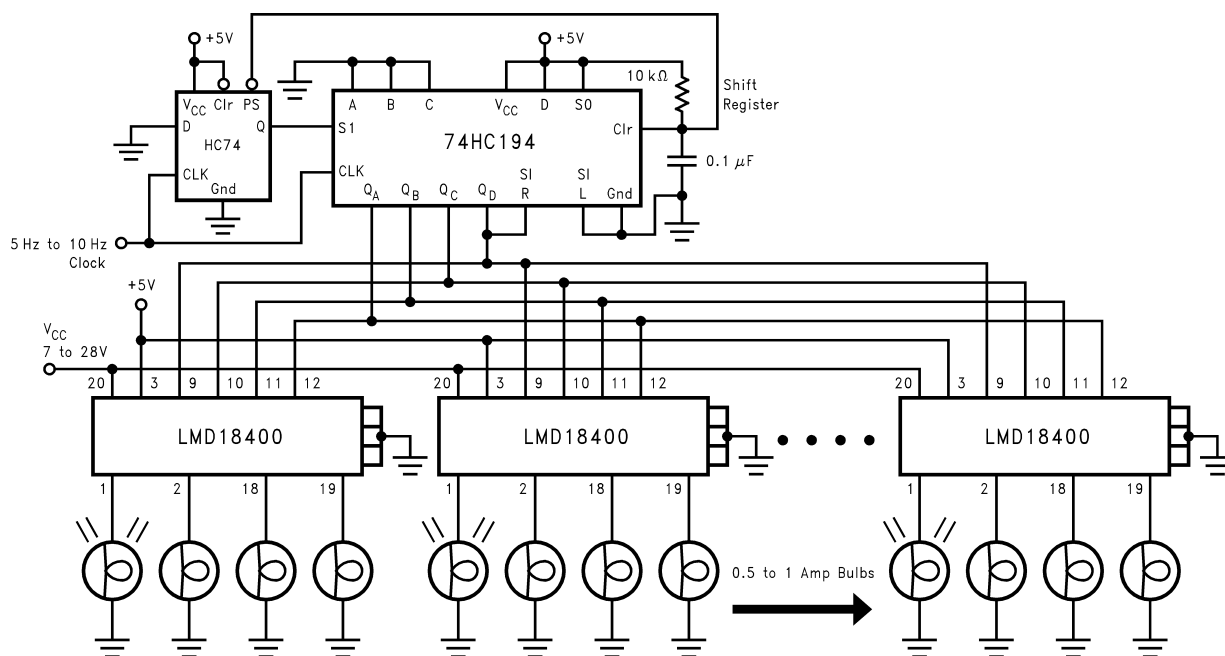
Figure 24. Simple Light "Chaser"
