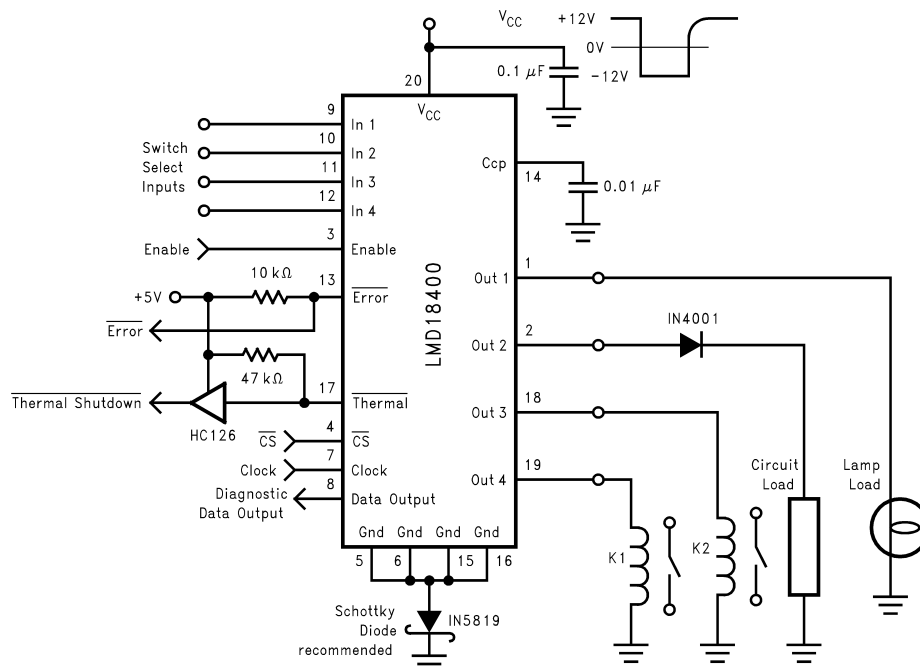
Figure 23. Simple protection of the LMD18400 against supply voltage reversal. Loads will be energized through the intrinsic diodes in parallel with the power switches. The Schottky diode will add approximately 0.2V to the logic input switching thresholds and the logic output low levels.
