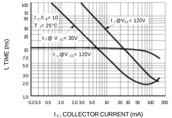
Figure 9. Turn-Off Time
