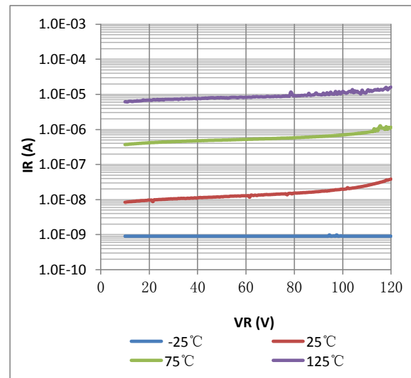
FIG.3 Reverse Characteristics
