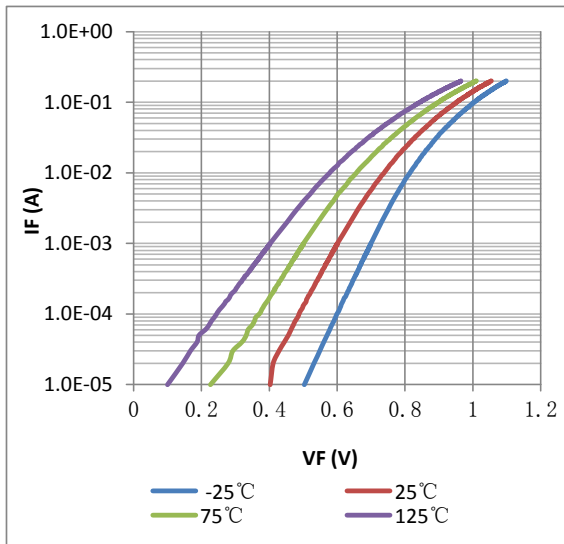
FIG.2 Forward Characteristics
