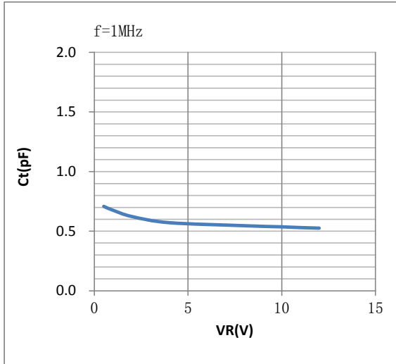
FIG.4 Capacitance
