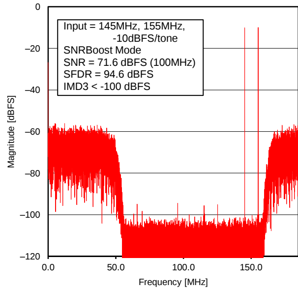
Figure 18. 2-Tone Spectrum (-10dBFS/tone, 145 & 155 MHz, F_C = 0.29 \cdot F_S )
