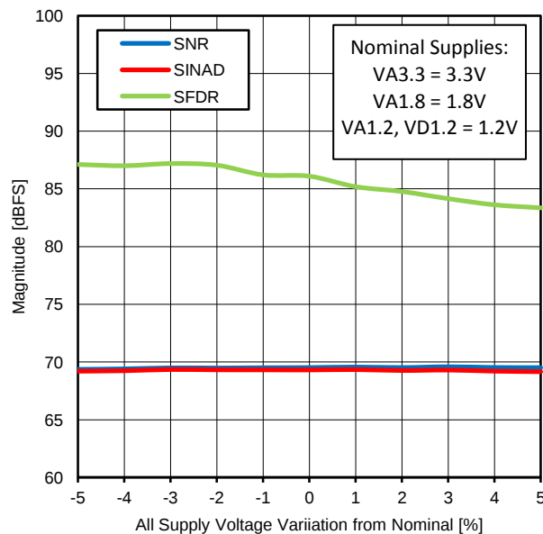
Figure 22. SNR, SINAD, SFDR vs. Supply
