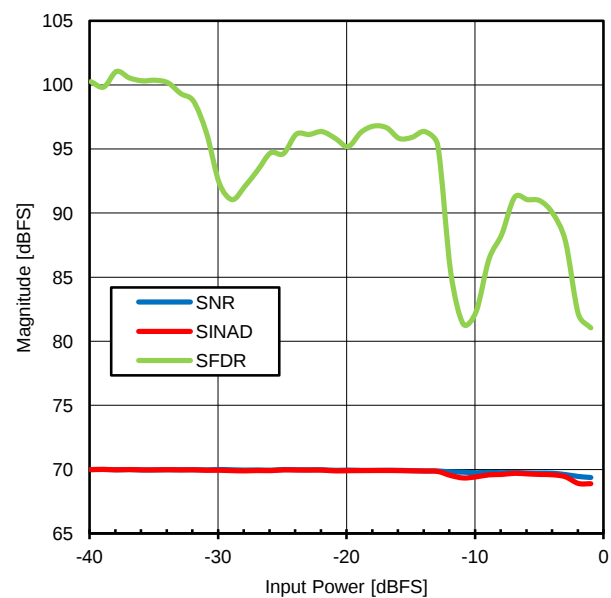
Figure 20. SNR, SINAD, SFDR vs. Input Power
