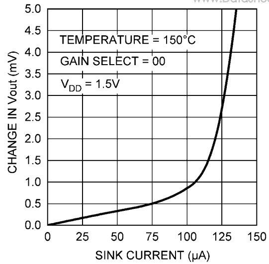
Load Regulation, Sinking Current
