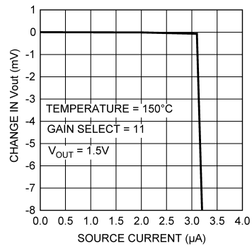
Load Regulation, Sourcing Current
