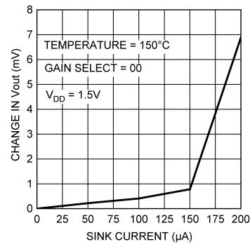
Load Regulation, Sinking Current
