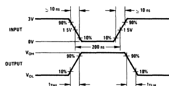
VOLTAGE WAVEFORMS
