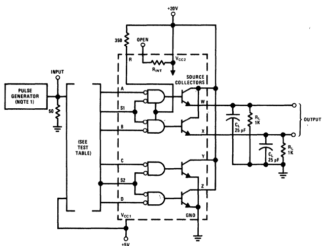
FIGURE 9. Switching Times
