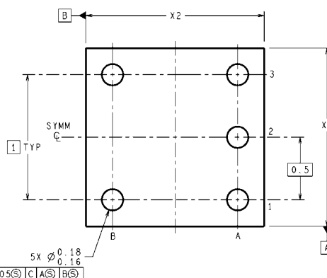
5-Bump micro SMD Ball Grid Array Thick Package Order Number LM74CIBP-3, LM74CIBPX-3, LM74CIBP-5, LM74CIBPX-5 NS Package Number BPD05MPB The following dimensions apply to the BPD05MPB package shown above: X1=1565µm ±30µm, X2=1615µm ±30µm, X3=850µm ±50µm.
