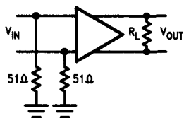
Test Circuit 1
