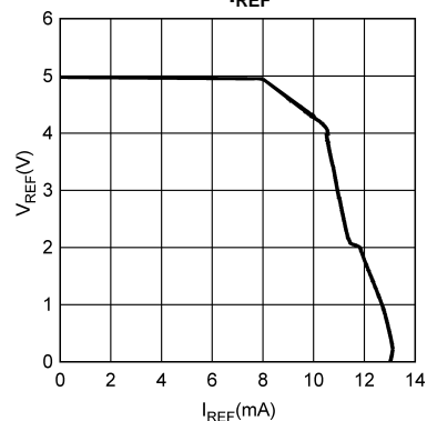
V_{REF} vs I_{REF}
