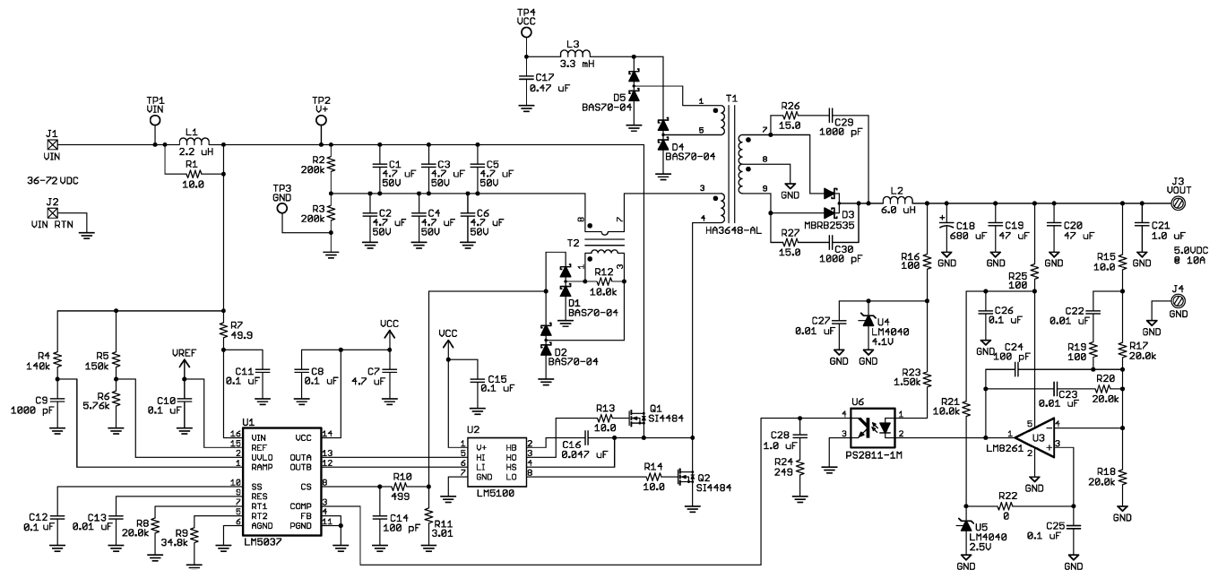
Figure 18. Schematic
