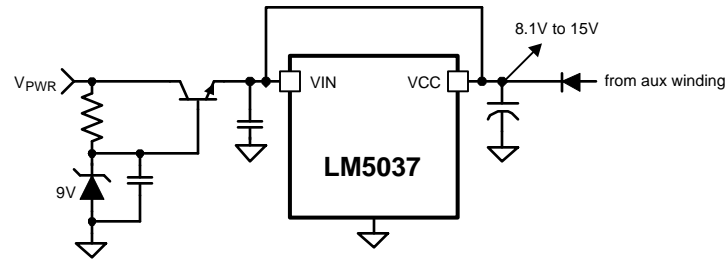
Figure 12. Start-up Regulator for VPWR >100V
