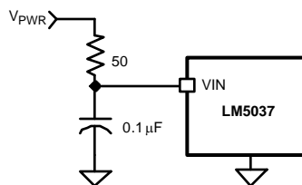
Figure 11. Input Transient Protection
