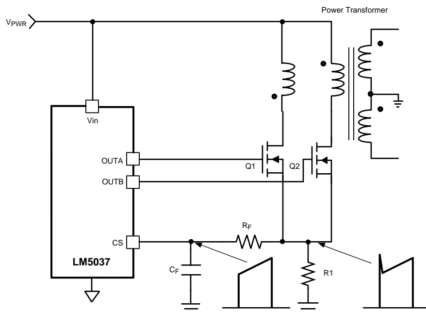
Figure 14. Current Sense Using Current Sense Resistor (R1)
