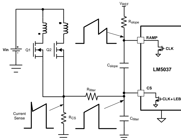
Figure 10. Current Mode Configuration
