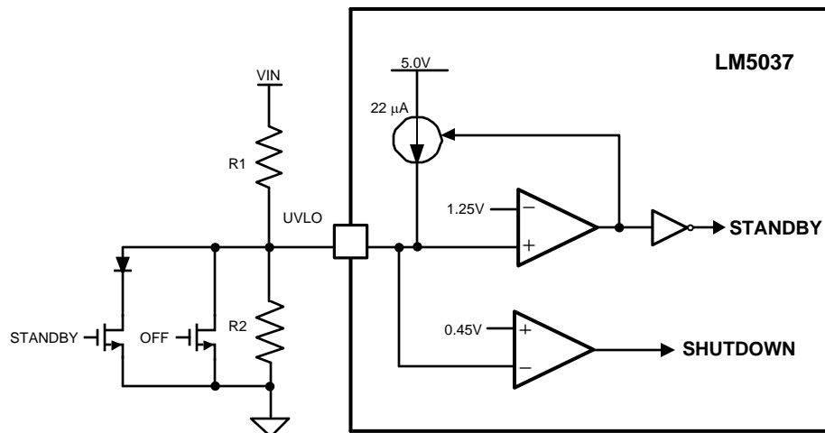
Figure 16. Remote Standby and Disable Control
