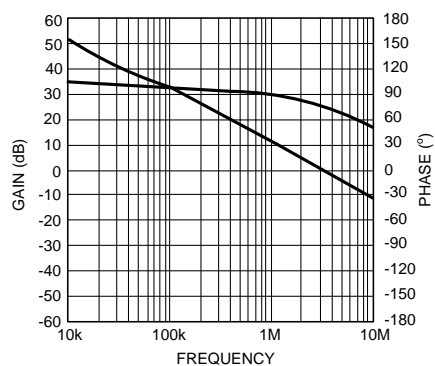
Feedback Amplifier Gain/Phase
