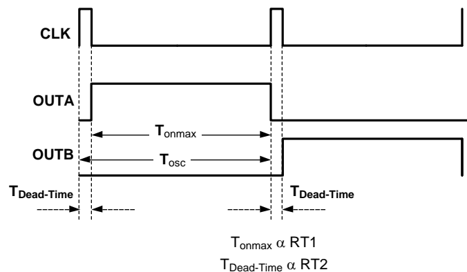
Figure 8. Timing Diagram of OUTA, OUTB and Dead-Time Set by RT2
