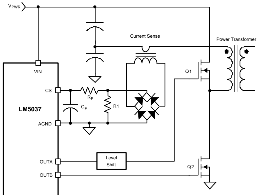
Figure 13. Current Sense Using Transformer
