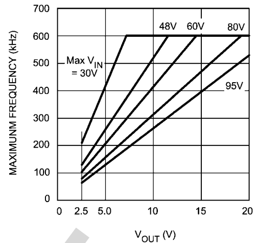
FIGURE 4. Maximum Frequency vs V_{OUT} and V_{IN}
