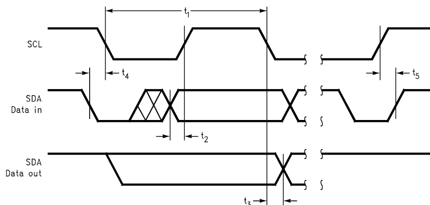
Figure 37. I 2 C Timing Diagram
