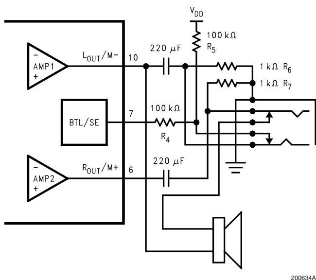
FIGURE 3. Headphone Operation and BTL - SE Mode Switching
