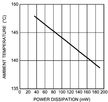
Power Derating Curve V_{DD} = 3V , R_L = 32\Omega
