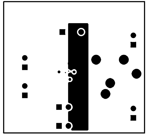
Midlayer 2
