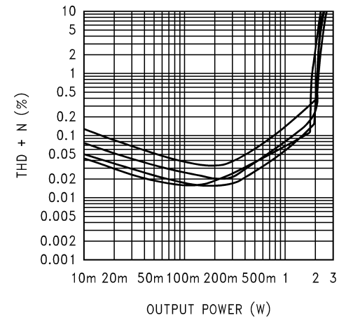
THD vs Output Power
