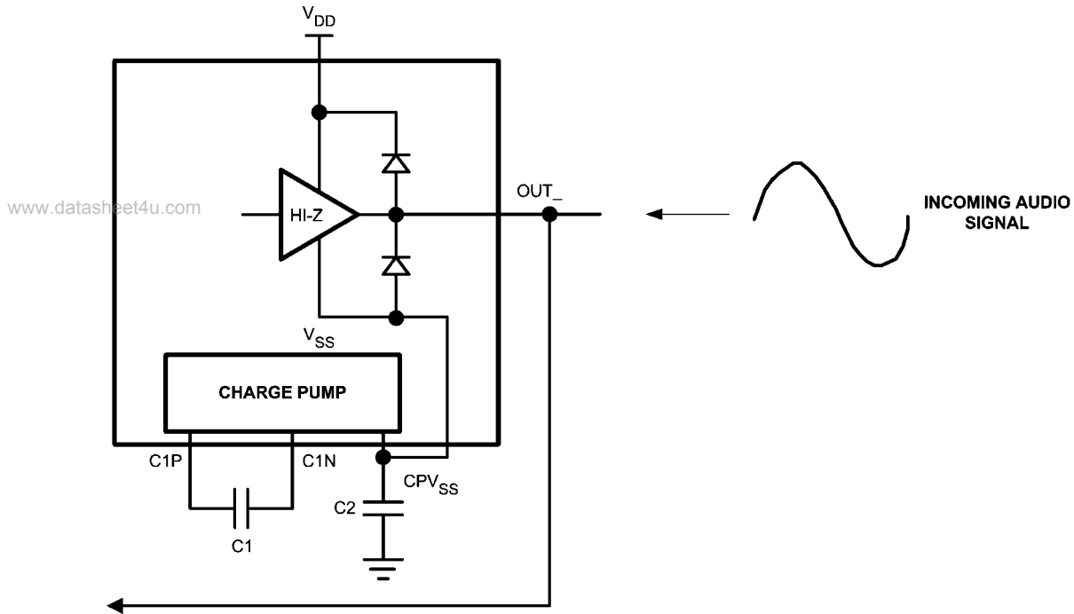
FIGURE 5. Back-Driving the LM48822 Outputs
