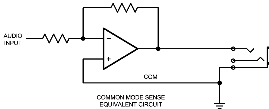
FIGURE 6. COM Connection Example
