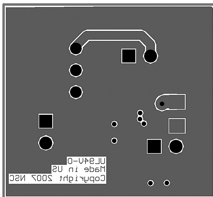
FIGURE 9: Bottom Layer
