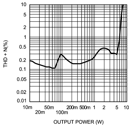
THD+N vs Output Power R_L = 8\Omega , V_{DD} = 12V , f = 1kHz
