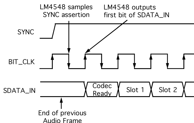
Figure 19. Start of Audio Input Frame
