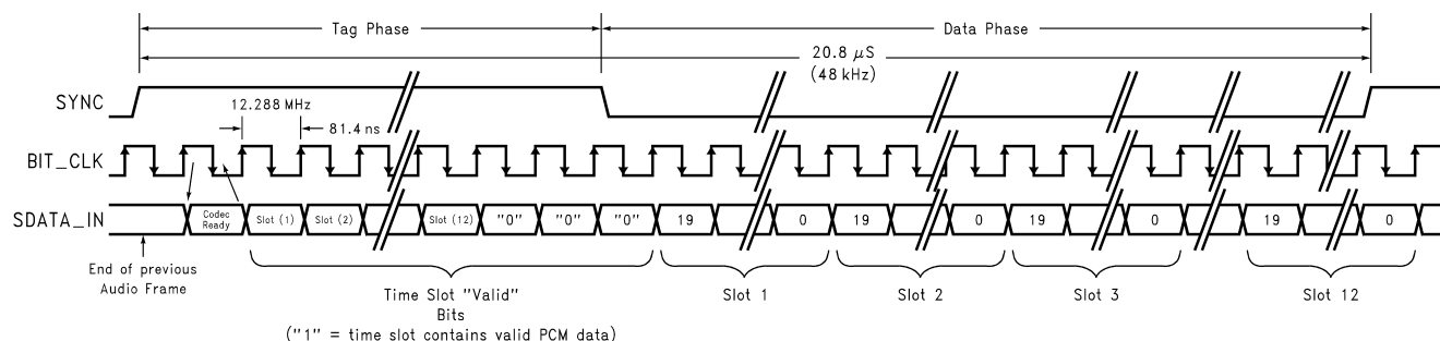
Figure 18. AC Link Audio Input Frame
