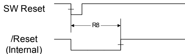
Figure 20-11. Software Reset Timing
