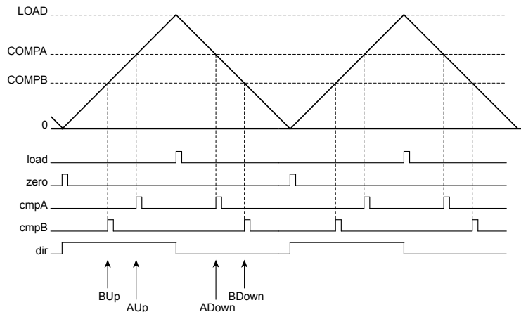
20.3.3 PWM Signal Generator
