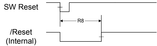
Figure 20-13. Watchdog Reset Timing
