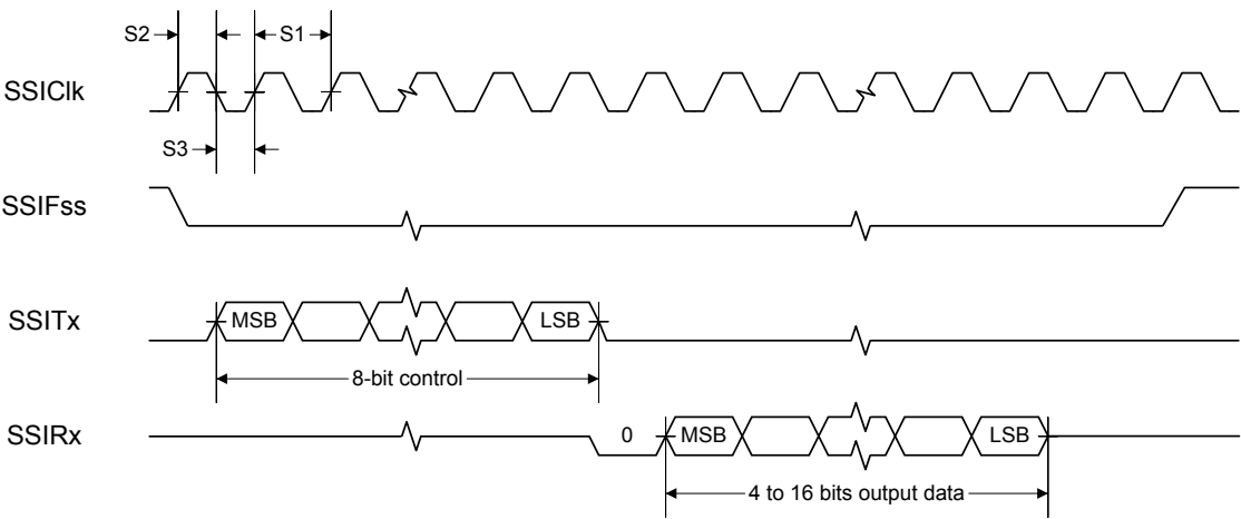
Figure 20-4. SSI Timing for MICROWIRE Frame Format (FRF=10), Single Transfer
