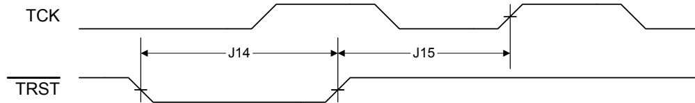
Figure 20-8. JTAG TRST Timing
