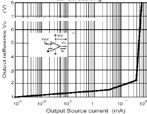
Fig.9 Output Characteristics current sourcing
