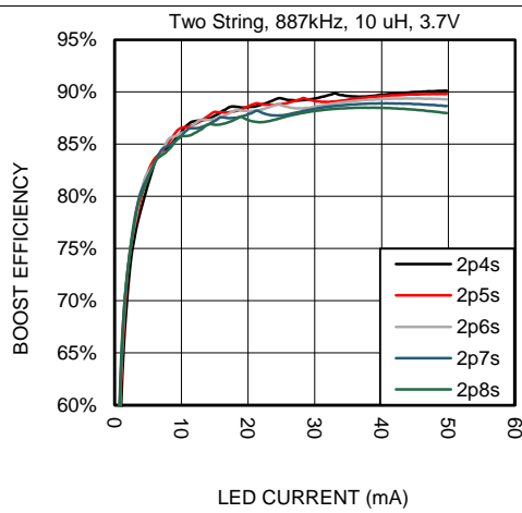
Figure 47. Boost Efficiency vs Series LEDs
