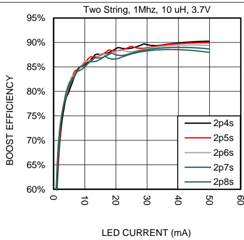
Figure 45. Boost Efficiency vs Series LEDs
