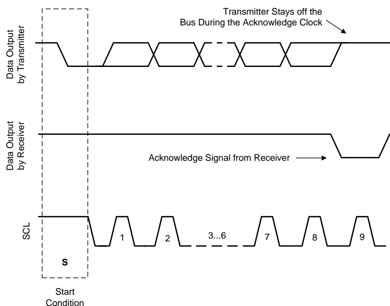
Figure 34. Acknowledge Signal
