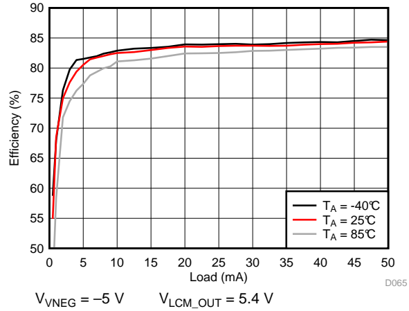
Figure 86. VNEG Efficiency
