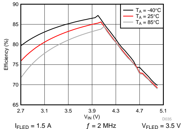
Figure 109. Flash System Efficiency
