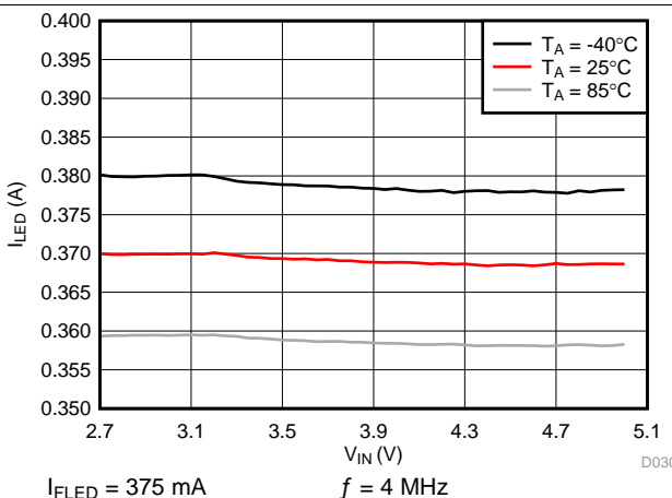
Figure 15. Flash LED Current
