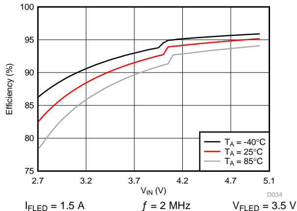
Figure 108. Flash Boost Efficiency
