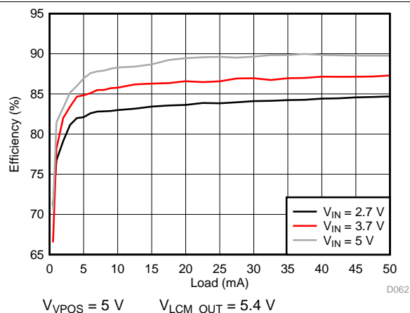
Figure 83. VPOS Efficiency
