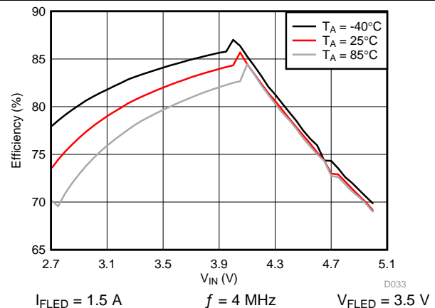
Figure 107. Flash System Efficiency
