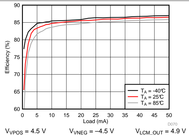
Figure 91. VPOS/VNEG Efficiency
