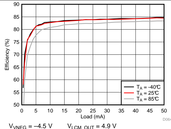
Figure 85. VNEG Efficiency
